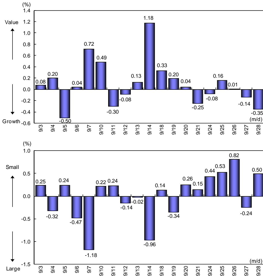
Fig. 7: Daily performance
